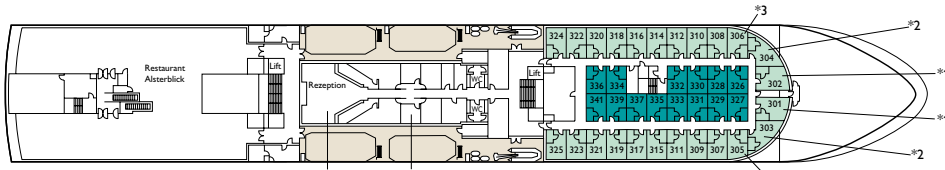
Deck 3
